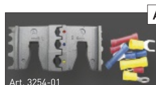
Art. 3254-01 DIN 0.5-1.0 / 1.5-2.5 / 4-6 mm 2 AWG 22-18 / 16-14 / 12-10
