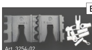
Art. 3254-02 DIN 1.5 / 2.5 / 6 / 10 mm 2 AWG 20-18 / 16-14 / 12-10 / 8 JIS 1.25 / 2 / 5.5 / 8 mm 2
